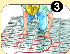
Install heating cable in grooves, pressing gently
